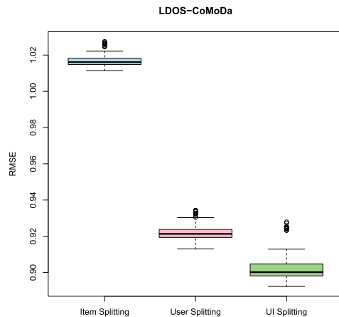
Figure 3: Boxplot of RMSE Among Splitting Approaches
