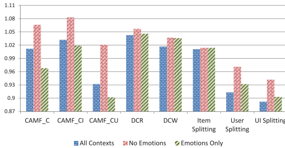
Figure 2: Comparison of RMSE Over Three Contextual Situations
