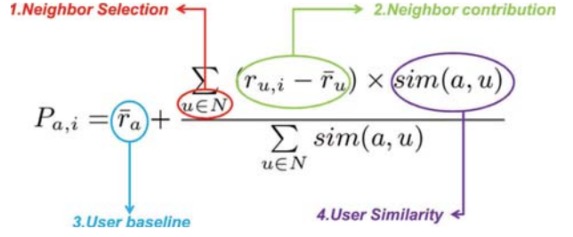
Figure 1: Algorithm Components in UBCF
